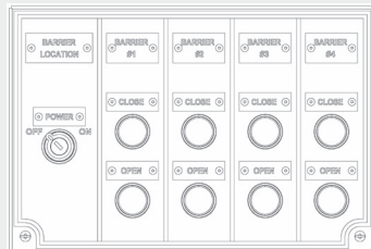
4-Barrier Control #SCP-1904
