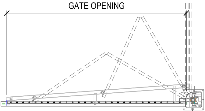
TOP VIEW: BI-FOLDING SWING GATE OUTSIDE LOOKING IN
