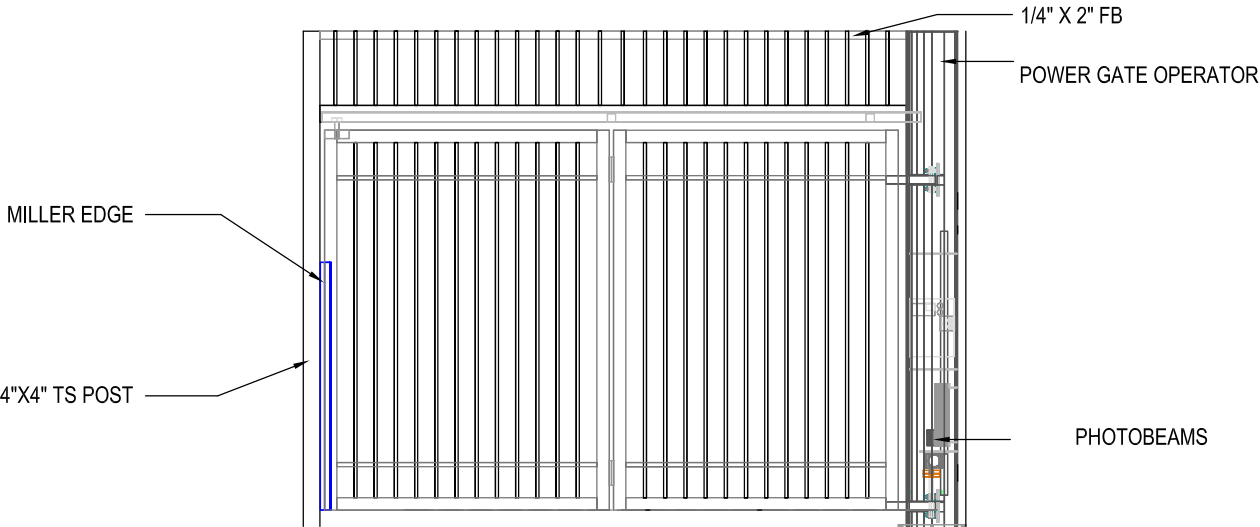
ELEVATION: BI-FOLDING SWING GATE OUTSIDE LOOKING IN
